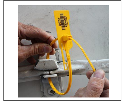
Art: BAGSEAL Plastic security seal. Flat tail with spikes. Ink transfer print Size : 6x420 mm
