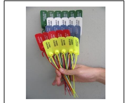
Art: JUPITER SEAL Plastic seal with metal closure. Round and smooth tail. With or without pre-cutting. Laser print. 2 x 315 mm 2 x 425 mm
