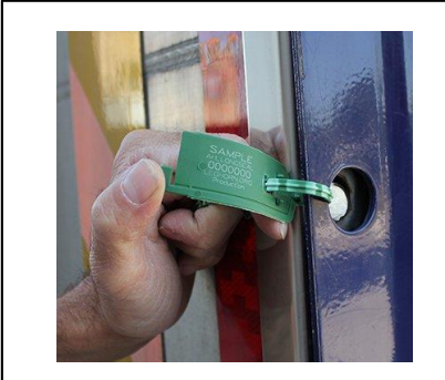
Art: LONGSEAL Plastic security seal. With pre-cutting. Laser print. Measures: 6x420 mm
