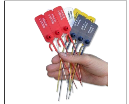
Art: JUPITER SEAL Plastic seal with metal closure. Laser print. 1,3x 325 mm With or without pre-cutting.
