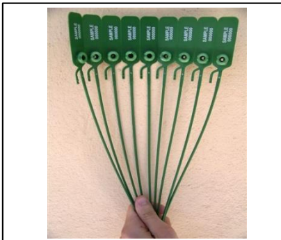
Art: JUPITER SEAL Plastic seal with metal closure. Laser print. 2 x 315 mm 2 x 425 mm With or without pre-cutting
