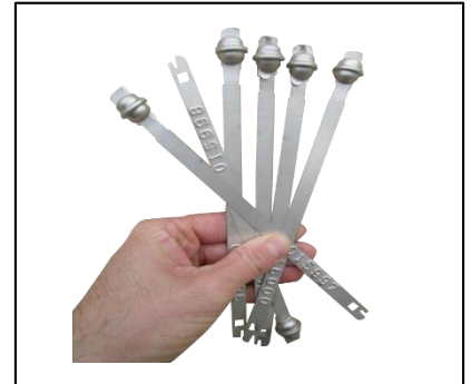
Art: METALSEAL Metal strap seal customisable and with progressive numbering in relief. Measures : 8x217 mm
